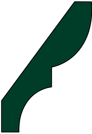
RM 70* 9/16 x 2 3/4
