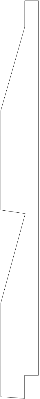
1 X 8 RMSP-149 FACE 6-5/8"
