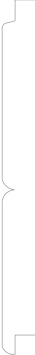
1 X 8 RMSP-150 FACE 6-3/4"
