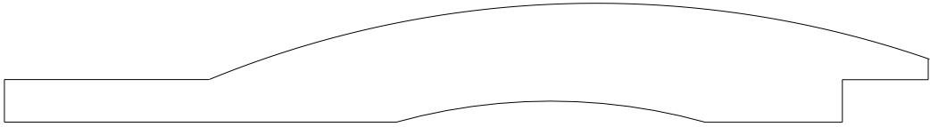
1 X 6 RMLS-406 FACE 4-7/8" REVEAL 3/4"
