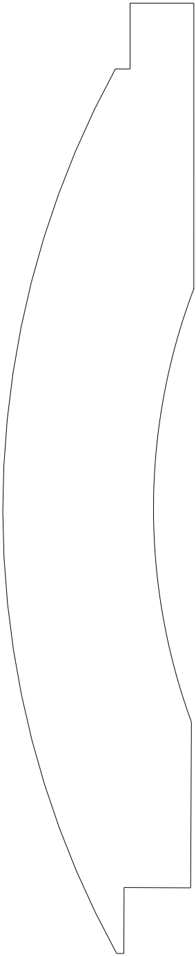
2 X 8 RMLS-441 FACE 6-5/8" NO REVEAL
