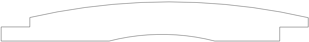
1 X 6 RMLS-407 FACE 4-7/8" NO REVEAL
