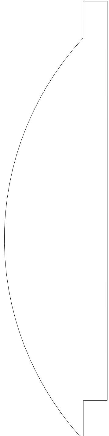
2 X 10 RMLS-443 FACE 6-3/4" REVEAL 1/8"
